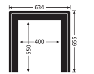
Optional inset steel fitting frame
