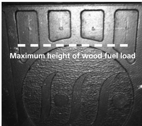
Maximum fuel load: This should never be higher than the lowest part of the logo circle in the tertiary air plate at the back of the firechamber as shown.
