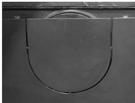
The Precision pre-cut rear heat shield. When using the rear flue outlet option the cut out can be easily removed by using a junior hacksaw blade to cut through the 3 small retaining links.
